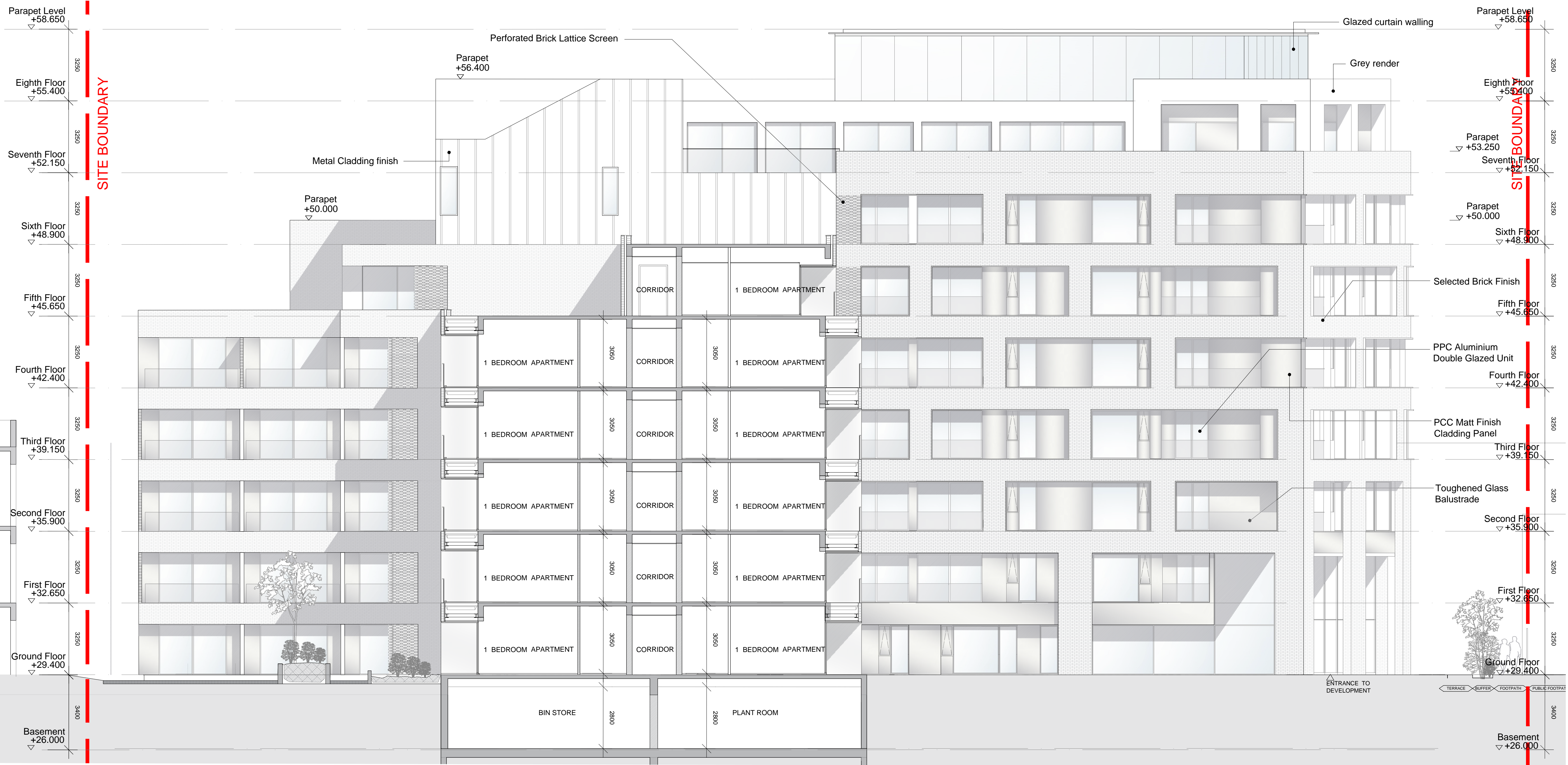
Section C-C - Scale 1:100@A1
